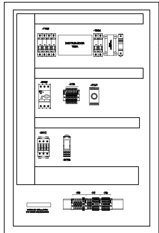
VISTA INTERIOR ARMARIO
